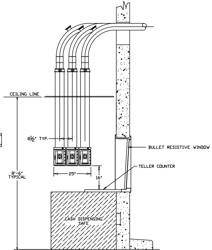
SECTION
